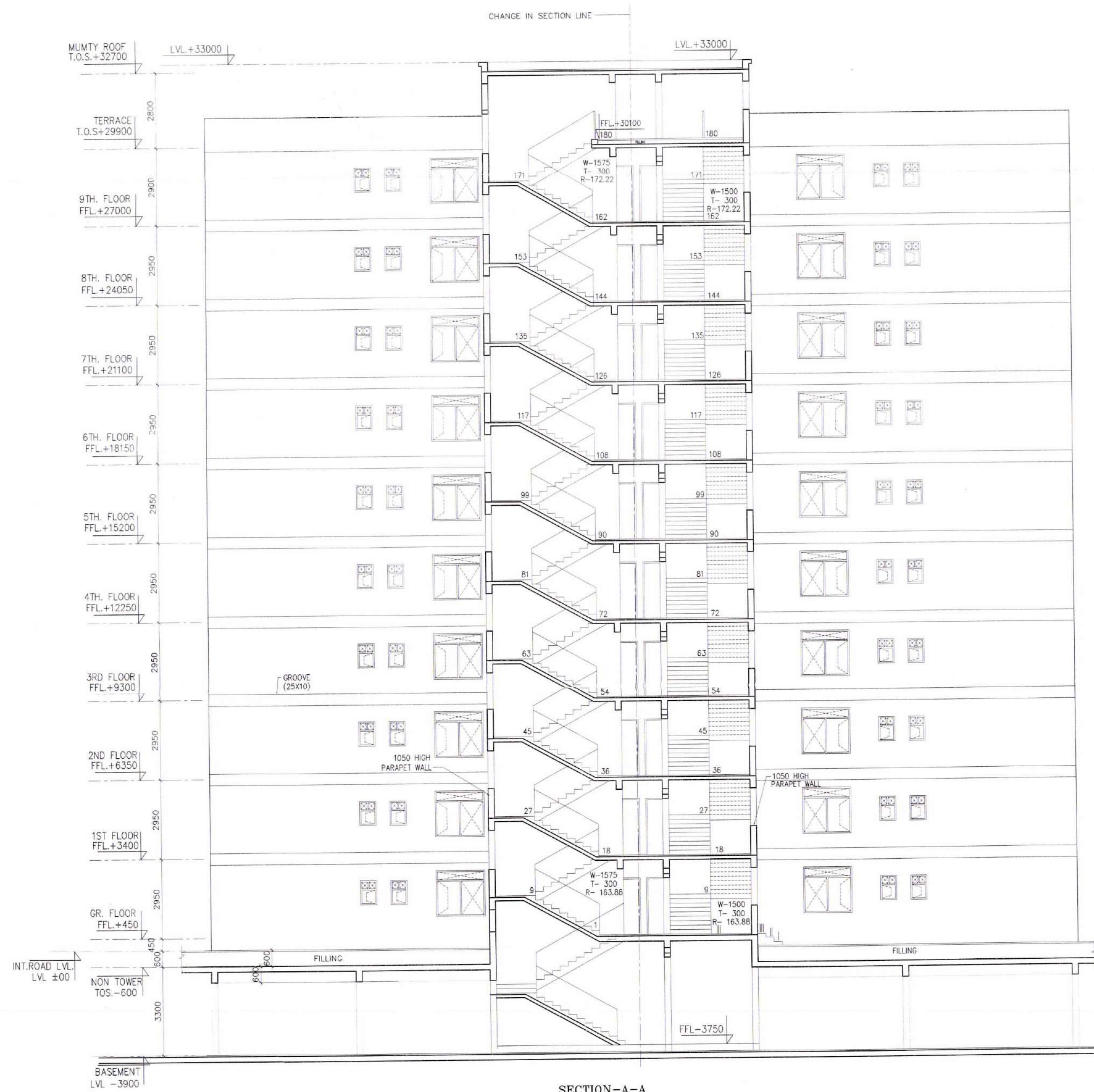
SECTION-A-A
